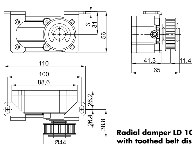
Radial damper LD 100 Z-Z26 with toothed belt disk Z26, without mounting bracket kit
