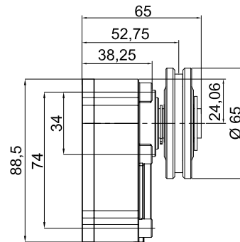
Radial damper LD 100 with rope pulley 65, without mounting bracket
