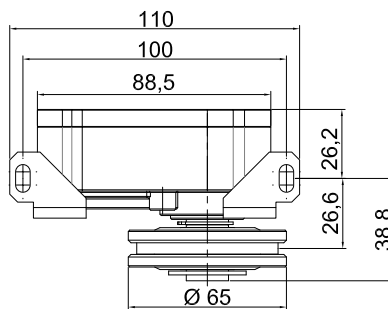
Radial damper LD 100 with rope pulley 65, with mounting bracket set
